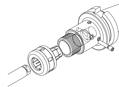
C-Lock弹簧夹头刀柄
